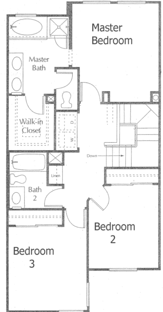
Second Floor
